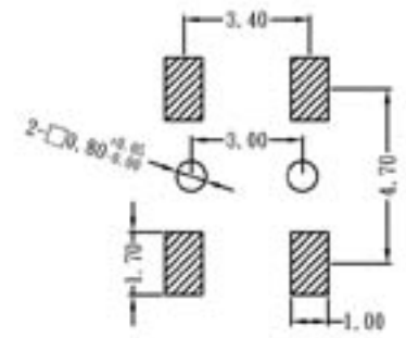
PCB DIMENSION
