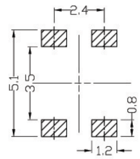
Pad Layout
