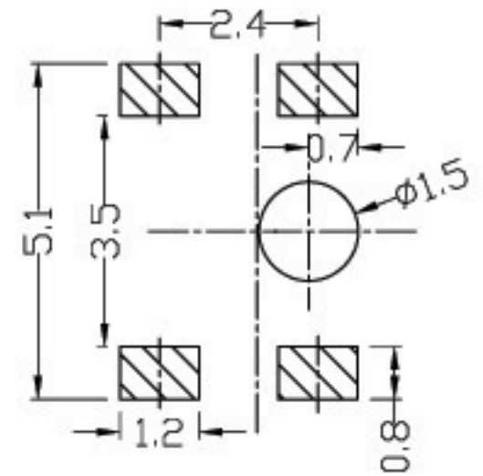
Pad Layout
