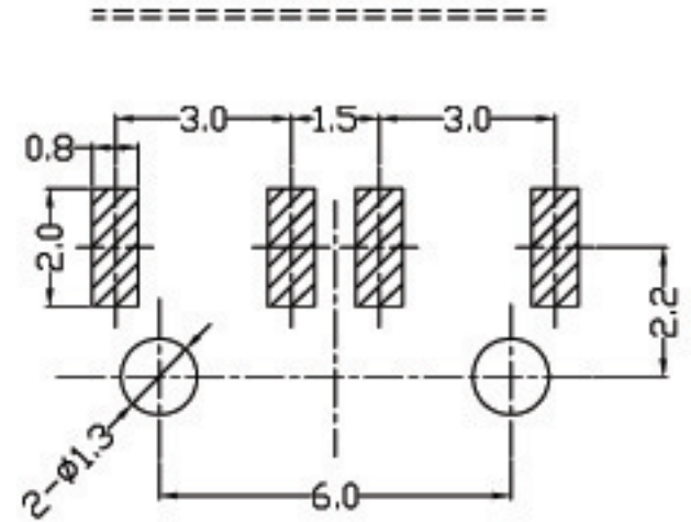
P.C.B. MOUNTING PATTERN
